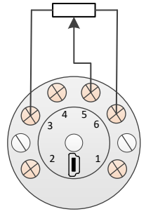
Slide Wire
