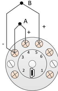
Dual Thermocouple
