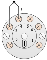
Thermocouple
