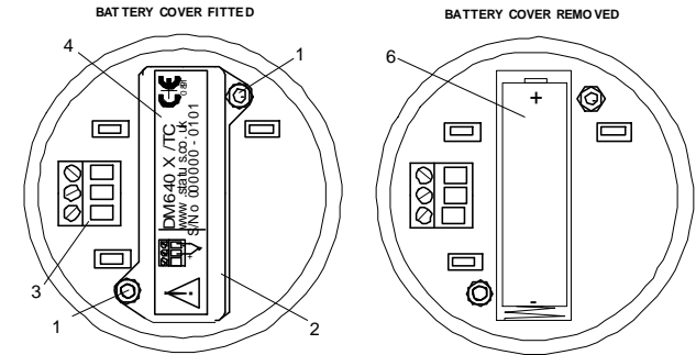
Fig 2 Rear view
