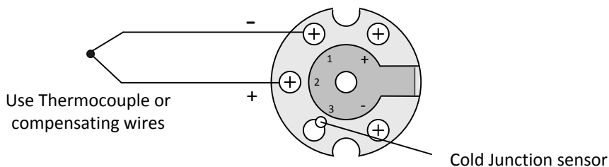
Thermocouple sensor connection
